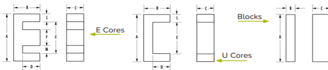
DIMENSIONS (mm)
